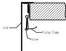
TOPMOUNT INSTALLATION
