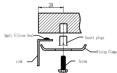
UNDERMOUNT INSTALLATION
